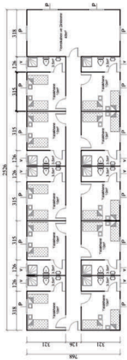
0 Prefabrik İdari Personel Yatakhane 194m 2 (20Kişilik) Prefabricated Staff Dormitory 194m 2 (20Person)
