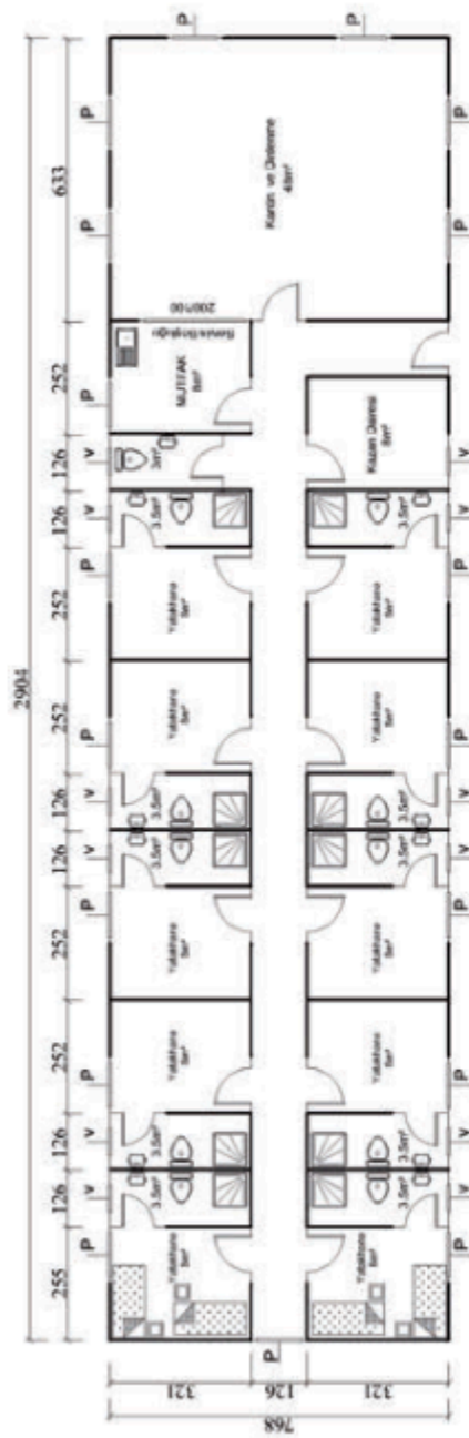
1 Prefabrik İdari Personel Yatakhane 223 m 2 (20 Kişilik) Prefabricated Staff Dormitory 223 m 2 (20 Person)
